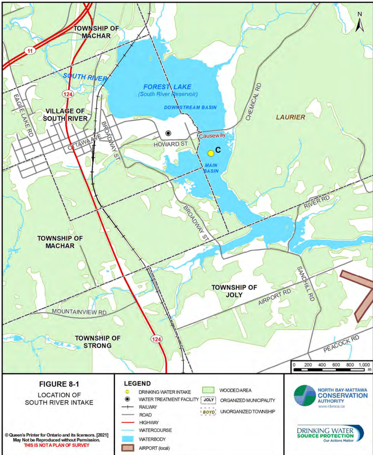
Figure 8-1. South River Intake
