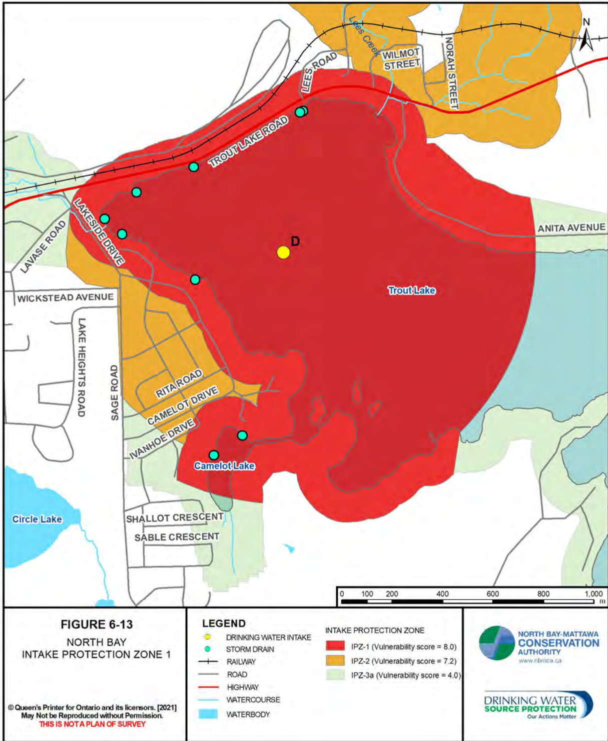
Figure 6-13. North Bay Intake Protection Zone-1
