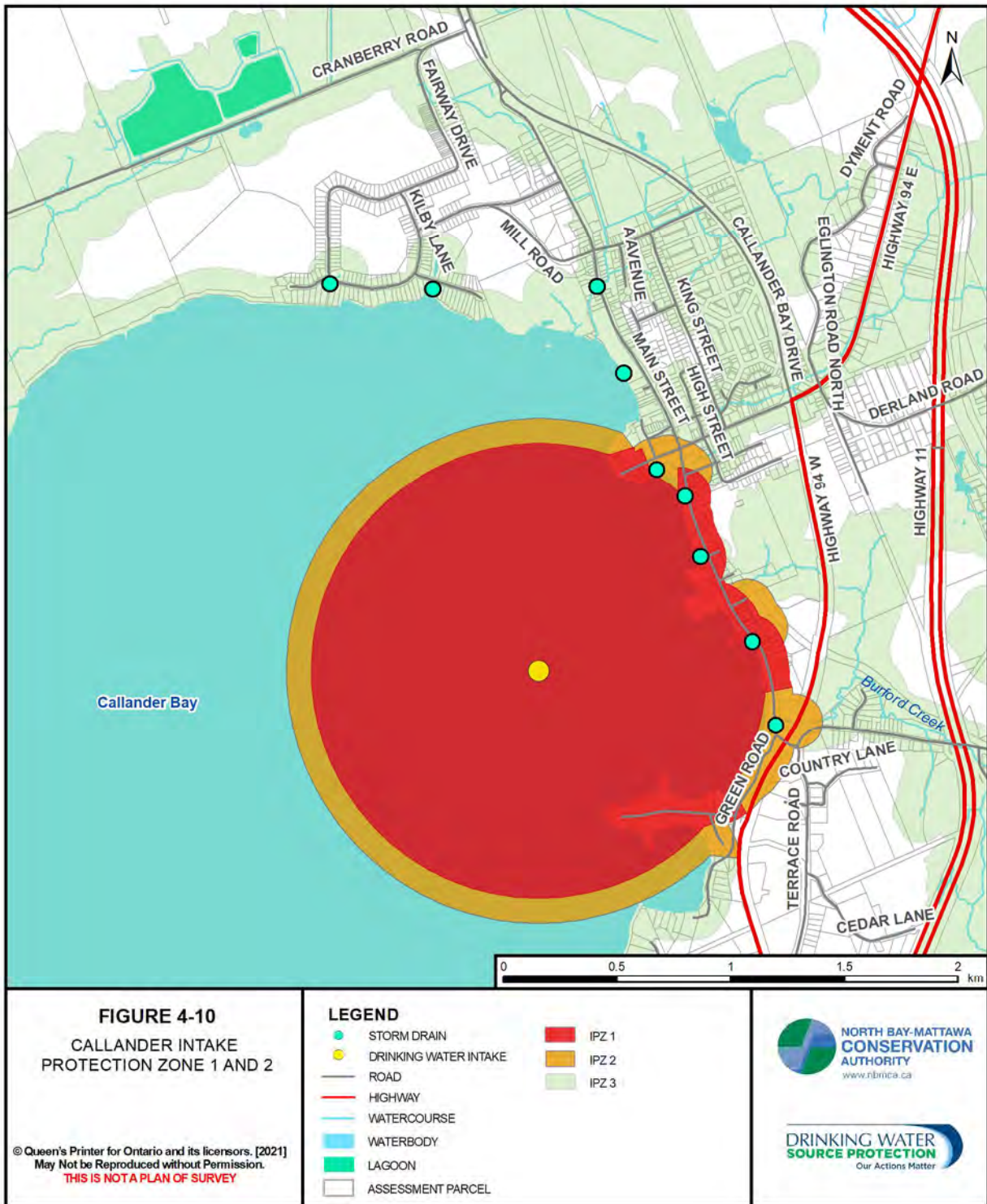
Figure 4-10. Callander Intake Protection Zone 1 and 2
