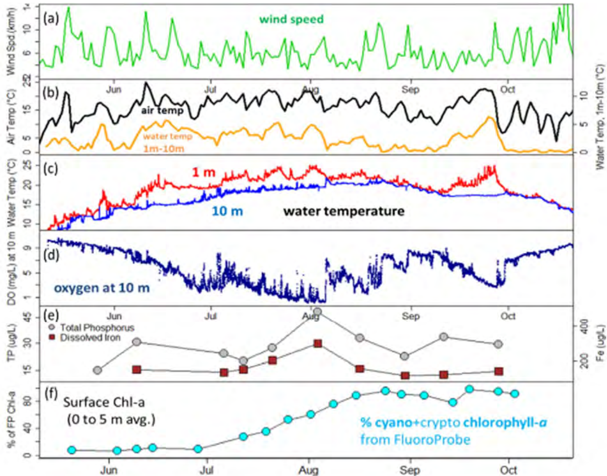
Figure 4-6. Water parameters in Callander Bay (2017)
