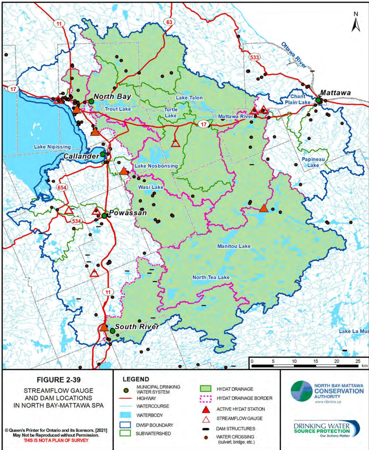
Figure 2-39. Streamflow Gauge Locations and Dam Structures
